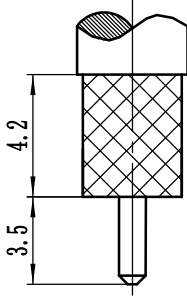
Recommended cable stripping dimensions
