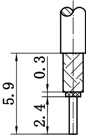
Recommended Cable Stripping Dimension
